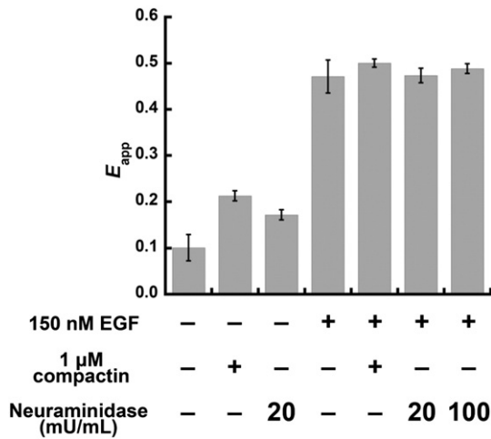
Fig. 3. E_{app} values after the depletion of cholesterol or monosialoganglioside GM3. All experiments were performed at X_D = 0.74 . Fluorescence spectra from EGF-stimulated CHO-K1 cells were observed 5–25 min after the EGF stimulation. Each value indicates the mean \pm SE. ( n > 10 ).
