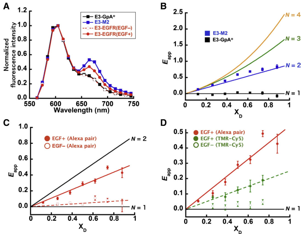
Fig. 2. Detection of the oligomeric states of membrane proteins by FRET. (A) Fluorescence spectra (Ex : 561 nm) from cell membranes labeled with the Alexa pair ( X_D = 0.5 ). Fluorescence spectra from at least 10 cells were averaged and normalized at 605 nm. Labeling conditions were the same as those described in Fig. 1. The symbols indicate a GpA G83I mutant (black squares), M2 proton channel (blue squares), EGFR without EGF (red open circles), and EGFR with 150 nM EGF (red solid circles). (B) Theoretical curves and measured E_{app} values at various donor mole fractions ( X_D ) using K4 probes labeled with the Alexa pair. Black, blue, green, and yellow lines show theoretical curves for monomers, dimers, trimers, and tetramers, respectively. N indicates the number of protomers in an oligomer. Black and blue squares indicate the E_{app} values for GpA* and M2, respectively ( n > 10 ). (C) The E_{app} values for EGFR with or without 150 nM EGF using K4 probes labeled with the Alexa pair. Open and solid circles indicate values in the absence and presence of EGF, respectively ( n > 10 ). The plots were linearly fit to obtain the slopes. (D) Comparison of E_{app} values for EGFR labeled with the Alexa pair (red) and the TMR-Cy5 pair (green). Open and solid symbols indicate values in the absence and presence of EGF, respectively ( n > 10 ).
