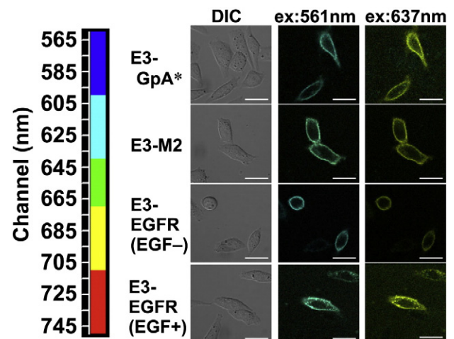
Fig. 1. Confocal images of E3-tagged proteins. Representative spectral images are shown in a pseudocolor. E3-tagged proteins were transiently expressed and labeled with a 1:1 mixture of a donor (Alexa568–K4) and acceptor (Alexa647–K4) ( X_D = 0.5 ) in PBS (+) (pH 7.4). The total K4 probe concentration was 100 nM (EGFRs) or 50 nM (the other proteins). All images were captured 5–25 min after labeling. GpA* as a standard of a monomer is the G83I mutant of glycoprotein A, which was derived from human erythrocytes. M2 as a standard of a dimer is the M2 proton channel derived from influenza A virus. Rat EGFRs were stimulated with 150 nM of rat EGF. Scale bar = 20 \mu m.
