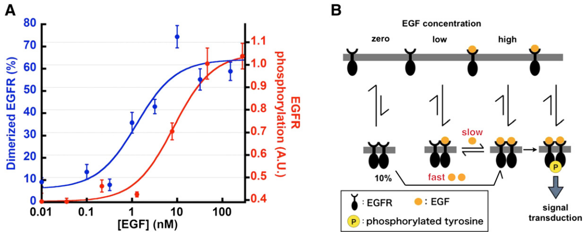
Fig. 5. EGF dose-dependent dimerization and phosphorylation of EGFRs. (A) The EGF concentration dependencies of EGFRs. Blue: Oligomerization 5–25 min after EGF stimulation. Red: Phosphorylation 5 min after EGF stimulation of EGFRs. The phosphorylation level was obtained from dot blotting (see Fig. A1, B). The dimer fraction was calculated from E_{app} values at X_D = 0.74 , assuming R = 56 Å. Each value indicates the mean \pm SE. ( n > 10 ). (B) Proposed model for the activation of EGFRs induced by EGF.
