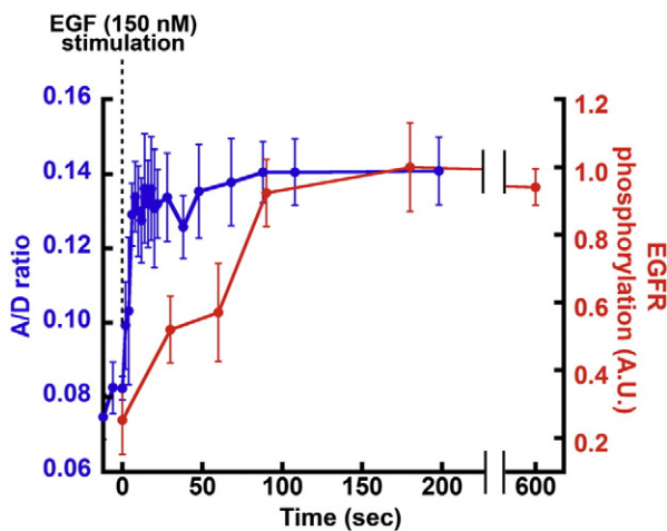
Fig. 4. Time courses of dimerization and phosphorylation upon stimulation. A/D is the ratio of the maximal fluorescence intensities of the acceptor (665 nm) to the donor (605 nm), which were obtained from the deconvoluted fluorescence spectra (Ex : 561 nm) of four cell membranes. Labeling was performed at X_D = 0.5 . The phosphorylation level was the relative chemiluminescence intensity for phosphorylated Tyr1173 to total EGFR as determined by dot blotting after the stimulation was stopped at each time point by the addition of the lyse buffer. The phosphorylation level was an average from three separately performed experiments. Each value indicates the mean \pm SE. ( n > 3 ).
